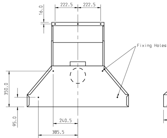
Rear View Showing Fixing Positions
